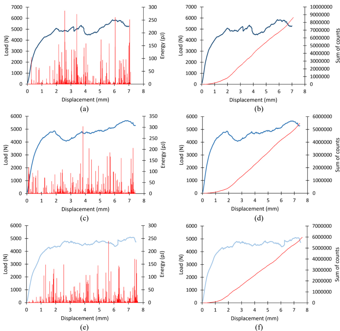
Figure 11. Load-displacement characteristics with AE signals: (a,b) specimen Sd-1x, (c,d) specimen Sd-2x, (e,f) specimen Sd-3x.
