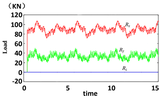
Figure 2. Load curve.
