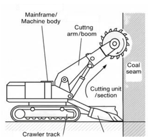
Figure 1. Schematic diagram of the continuous miner.
