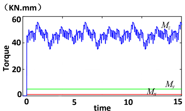
Figure 2. Load curve.
