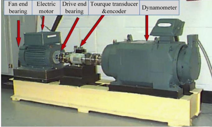
Figure 6. Physical Structure of the CWRU Test Bench.
