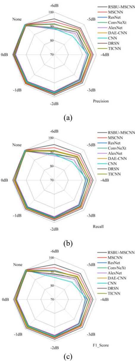
Figure 10. Radar chart of the three evaluation metrics under the CWRU dataset. (a) Precision (b) Recall (c) F1_Score.
