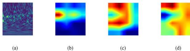
Figure 14. Grad-CAM visualization of scale-specific feature responses under noisy vibration signals. (a) input (b) 3×3 branch (c) 5×5 branch (d) 7×7 branch.
