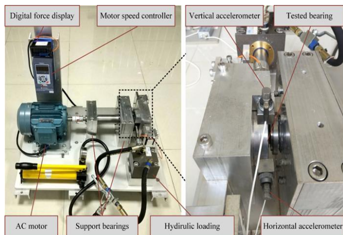
Figure 16. Physical structure of the XJTU-SY test bench.
