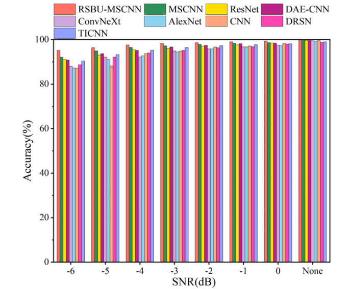
Figure 9. Bar chart of test accuracy for the CWRU dataset.
