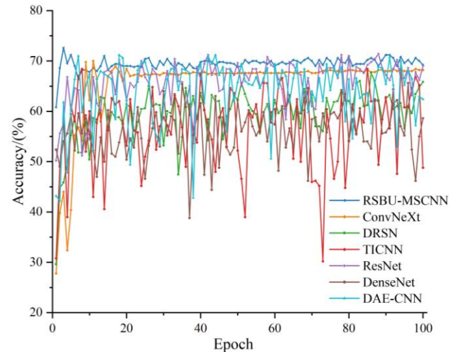
Figure 24. Cross-SNR Generalization Test ( -6 dB \rightarrow -10 dB).
