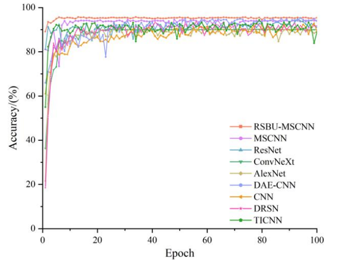
Figure 8. Accuracy curve at SNR = -6 dB.
