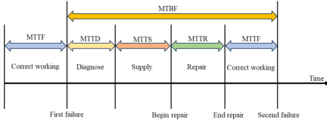
Fig. 4. A schematic diagram of MTTF, MTTD, MTTS, MTTR, and MTBF.
