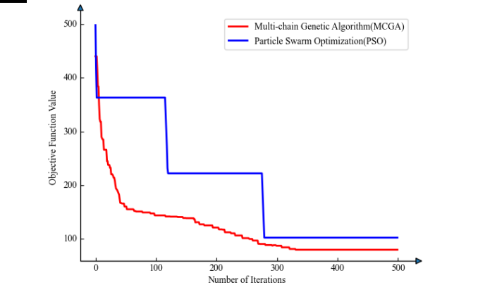
Fig.4. Iterative curve of fitness values.
