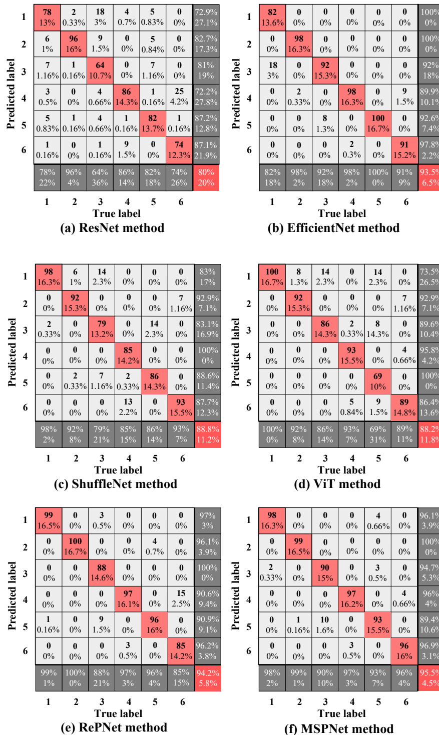
Fig. 7. Confusion matrix for different methods.
