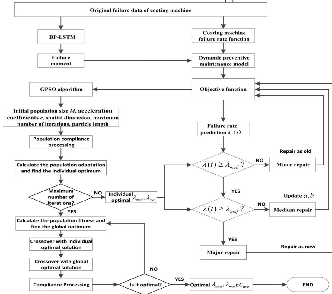
Fig. 7. Flow chart of dynamic preventive maintenance model solving based on GPSO algorithm.
