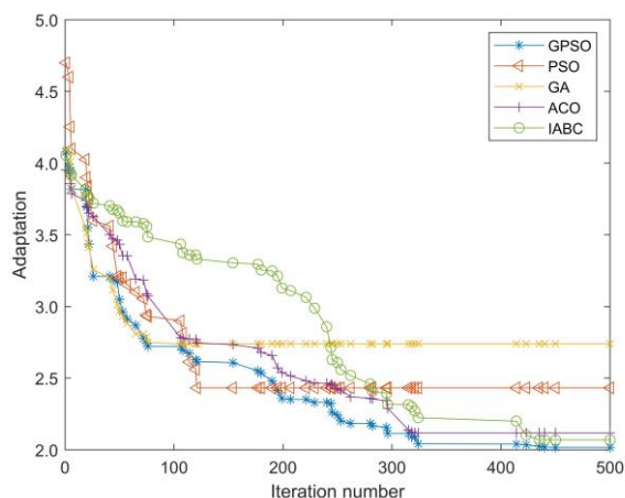
Fig. 11. Comparison of optimal adaptation of five algorithms.
