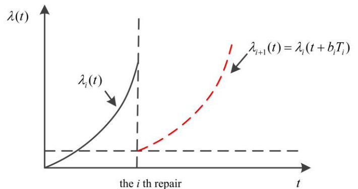
Fig. 3. Failure rate evolution rule with service age decrement factor.
