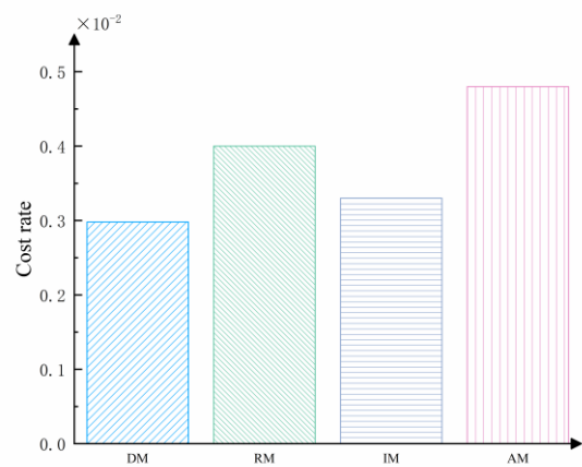
Fig. 10. Dynamic preventive maintenance model compared with other maintenance models cost rate.
