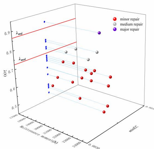
Fig. 13. Future 6500h maintenance strategy chart for coating machine.
