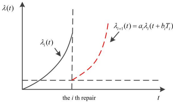
Fig. 4. Evolution rule of failure rate with two adjustment factors.
