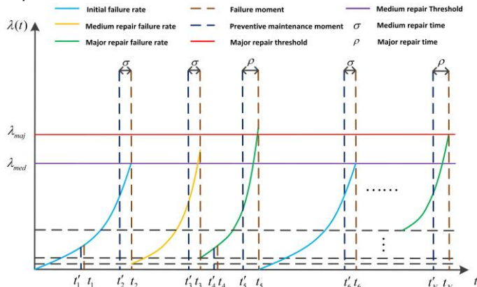
Fig. 1. Three maintenance modes of dynamic preventive maintenance strategy for coating machine.
