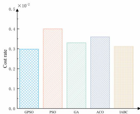
Fig. 12. Comparison of five algorithm cost rate.
