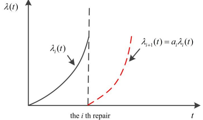
Fig. 2. Failure rate evolution rule with increasing failure rate factor.
