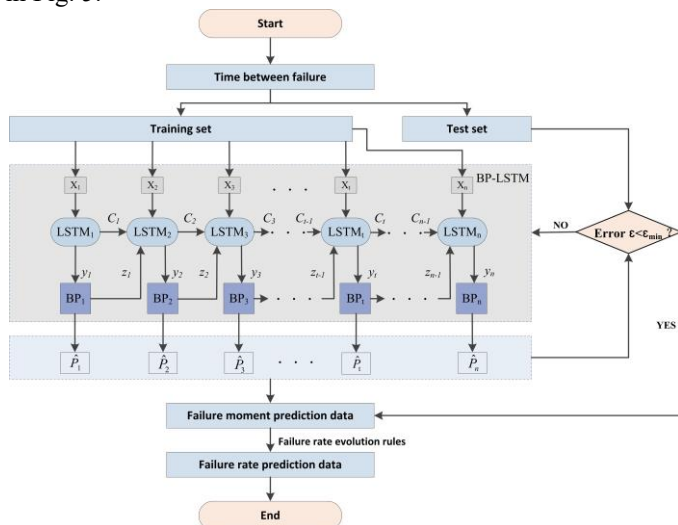
Fig. 5 Failure rate prediction framework based on BP-LSTM.
