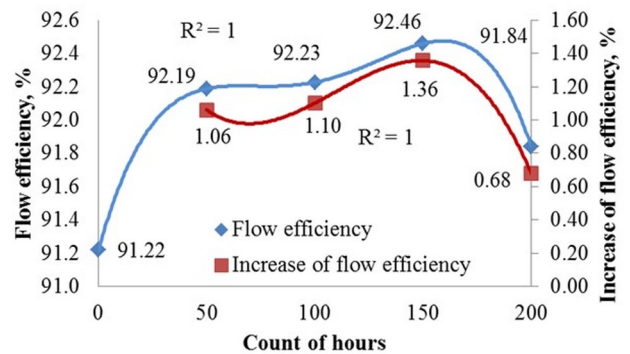
Fig. 6. Flow efficiency and increase of the flow efficiency at pressure p = 10 MPa
