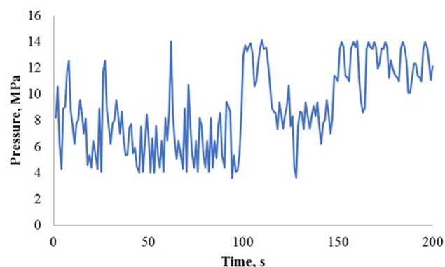
Fig. 1. Operational characteristics of the loading of the hydraulic pump
