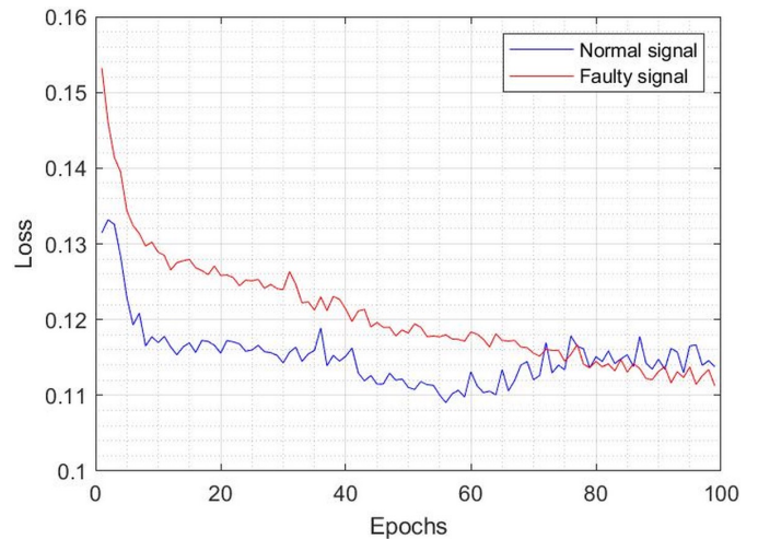
Fig. 12. Model learning loss for successive iterations
