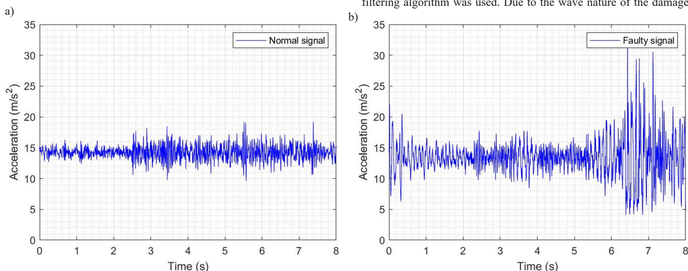
Fig. 4. Acceleration of transverse vibrations along the length of the laboratory conveyor: a) without damaged roller, b) with damaged roller
