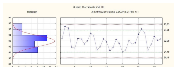
Fig. 9. \bar{X} card for the 250 Hz octave spectrum
