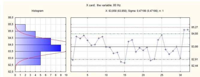
Fig. 21. \bar{X} card for the 80 Hz 1/3 octave spectrum
