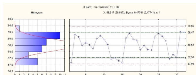
Fig. 17. \bar{X} card for the 31,5 Hz 1/3 octave spectrum
