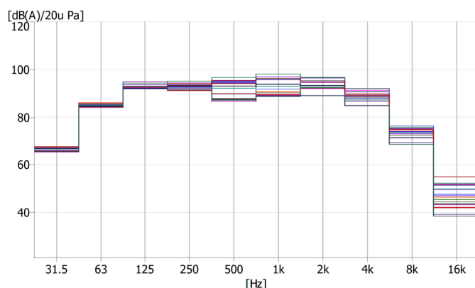
Fig. 5. Octave spectra of the acoustic signals
