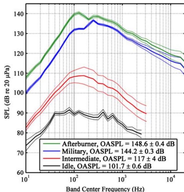
Fig. 1. 1/3 octave spectra measured along the reference array at z=15.2 m. Solid lines represent the SPL values averaged over all scans [56]
