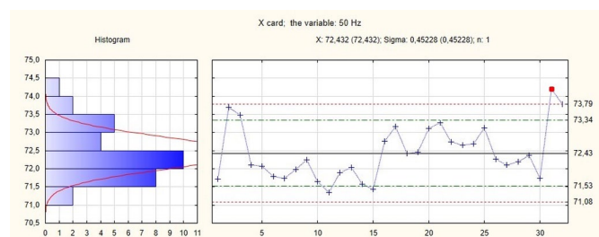
Fig. 19. \bar{X} card for the 50 Hz 1/3 octave spectrum
