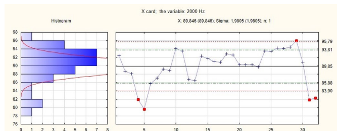
Fig 35. \bar{X} card for the 2000 Hz 1/3 octave spectrum
