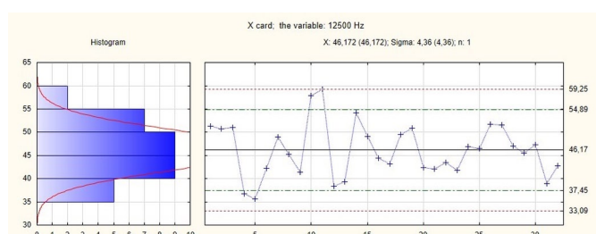
Fig 43. \bar{X} card for the 12500 Hz 1/3 octave spectrum
