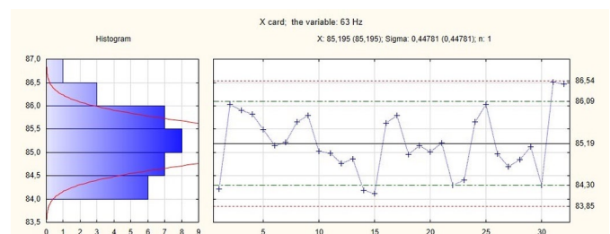
Fig. 7. \bar{X} card for the 63 Hz octave spectrum
