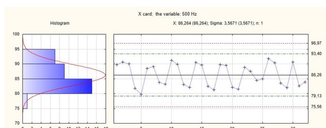
Fig. 29. \bar{X} card for the 500 Hz 1/3 octave spectrum
