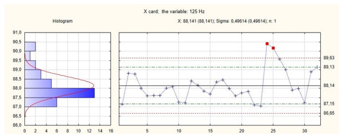
Fig. 23. \bar{X} card for the 125 Hz 1/3 octave spectrum
