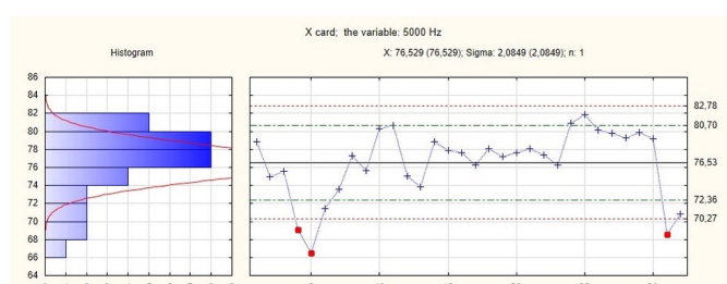
Fig 39. \bar{X} card for the 5000 Hz 1/3 octave spectrum
