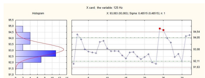
Fig. 8. \bar{X} card for the 125 Hz octave spectrum
