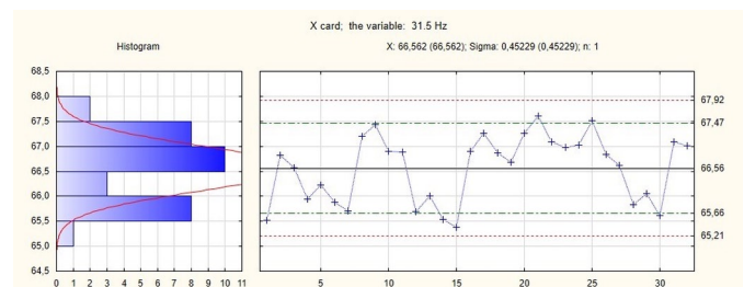
Fig. 6. \bar{X} card for the 31,5 Hz octave spectrum
