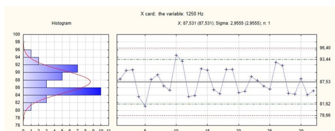
Fig. 33. \bar{X} card for the 1250 Hz 1/3 octave spectrum
