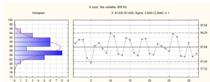
Fig. 31. \bar{X} card for the 800 Hz 1/3 octave spectrum
