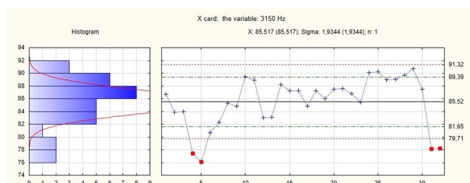
Fig 37. \bar{X} card for the 3150 Hz 1/3 octave spectrum
