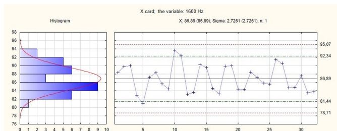
Fig 34. \bar{X} card for the 1600 Hz 1/3 octave spectrum
