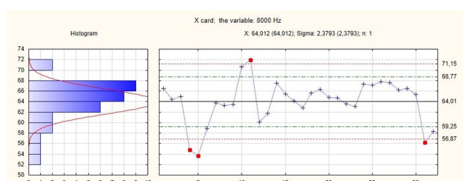
Fig 41. \bar{X} card for the 8000 Hz 1/3 octave spectrum
