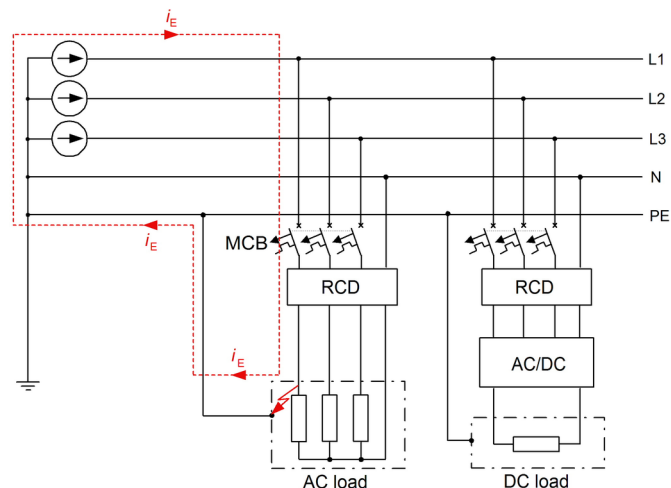
Fig. 2. The structure of low-voltage AC 230/400 V installation, and the flow of earth fault current i_E in the case of insulation-to-earth fault in AC load. MCB – overcurrent protection device (miniature circuit breaker), RCD – residual current device
