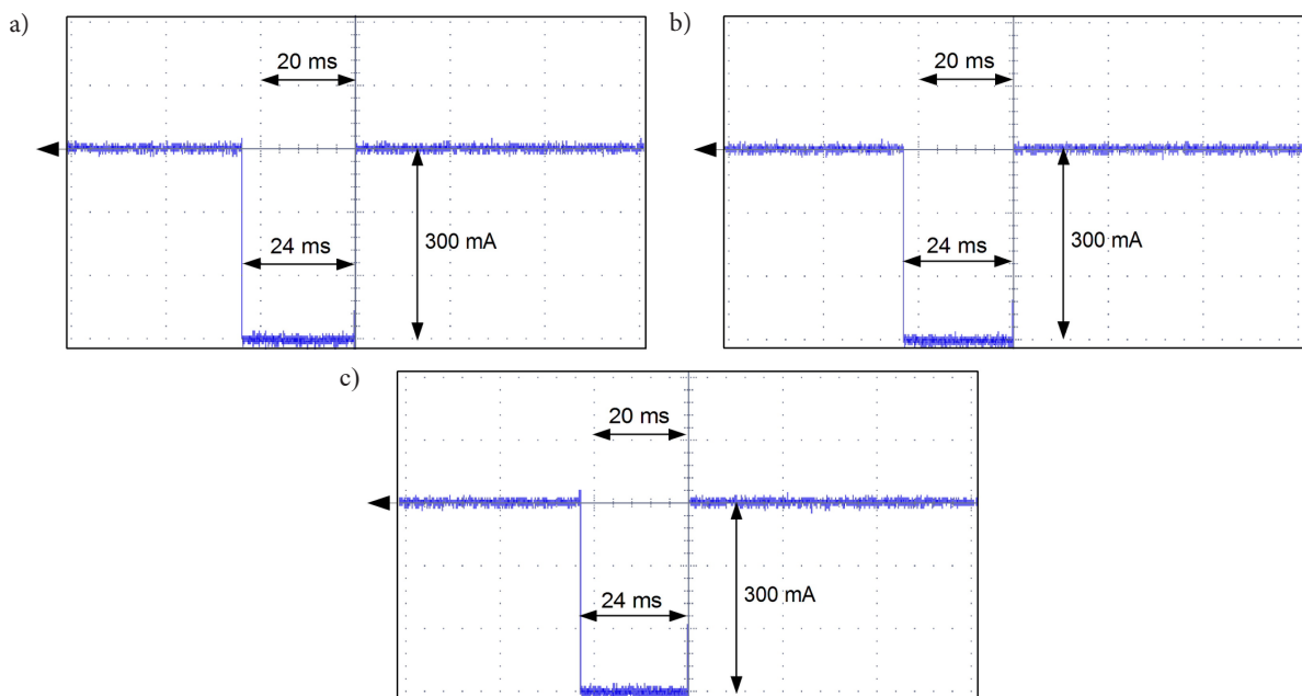
Fig. 13. Residual current oscillograms during the operation of 30 mA RCD-B3 under the suddenly applied DC residual current of 300 mA: a) AC 230 V auxiliary voltage used (poles L-N), b) DC 230 V auxiliary voltage used (poles L-N), c) no auxiliary voltage used
