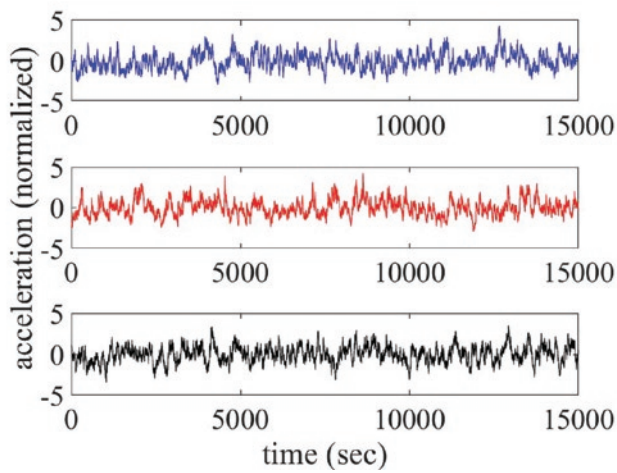
Fig. 4. Normalized acceleration time series obtained from the x-axis for the selected clearance of RIC=20 \mu\text{m} – blue, 22 \mu\text{m} – red and 34 \mu\text{m} – black
